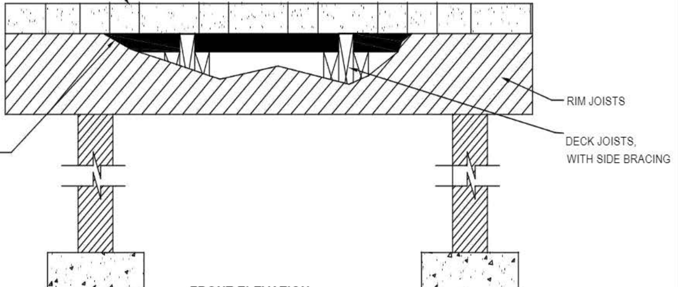
FRONT ELEVATION
